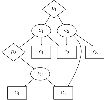
Fig. 2. A MulVAL proof graph
