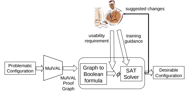
Fig. 1. SAT-based configuration generation
