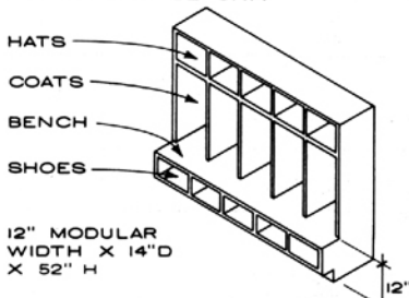
12" MODULAR WIDTH X 14" D X 52" H LOCKER UNIT
