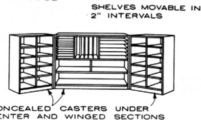
46" W (CLOSED) X 14" D X 34" H FOLDING STORAGE UNIT
