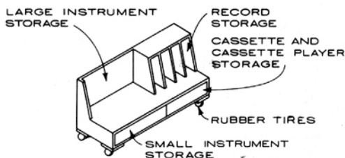
54" W X 18" D X 28" H MUSIC CART
